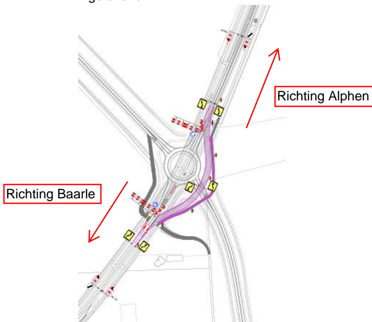
Figure 1 Schets bypass rotonde Alphenseweg
